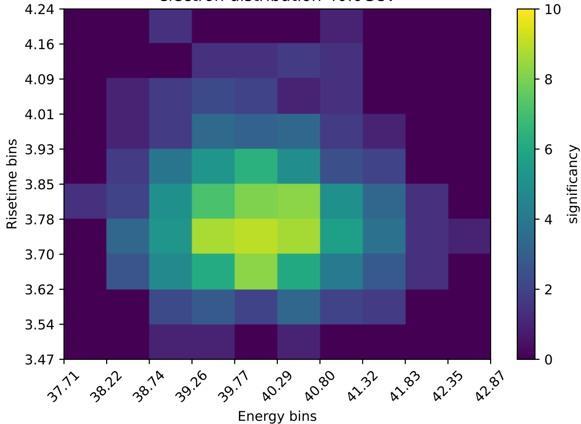
electron distribution 40.0GeV
